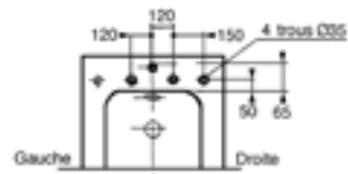
PERCEMENT 77 - robinetterie 4 trous Ø 35
