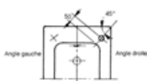
PERCEMENT 09 - robinetterie 1 trou Ø 35
