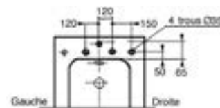
PERCEMENT 77 - robinetterie 4 trous Ø 35
