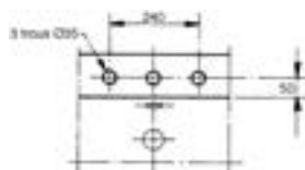
PERCEMENT 04 - robinetterie 3 trous Ø 35 - 240 mm
