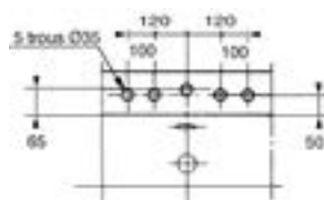
PERCEMENT 25 - robinetterie 5 trous Ø 35
