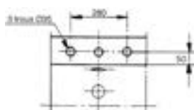
PERCEMENT 05 - robinetterie 3 trous Ø 35 - 280 mm
