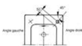
PERCEMENT 09 - robinetterie 1 trou Ø 35
