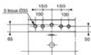
PERCEMENT 23 - robinetterie 5 trous Ø 35
